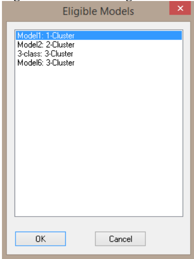
Figure 7-24. List of Eligible Reference Models for Conditional Bootstrap
