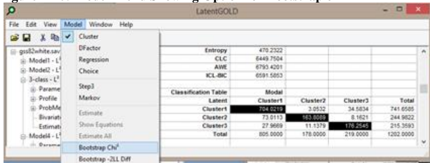
Figure 7-10: Model Menu Showing Option for Bootstrap of L 2
