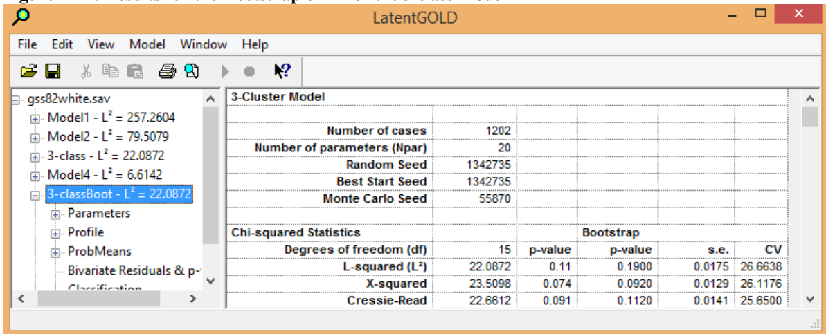
Figure 7-11: Results for the Bootstrap of L 2 for the 3-class Model
