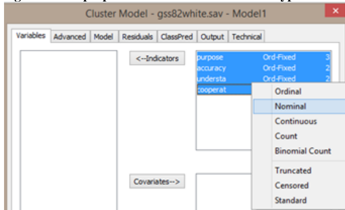
Figure 7-7. Pop-up Menu to Set Variable Scale Types and Subtypes
