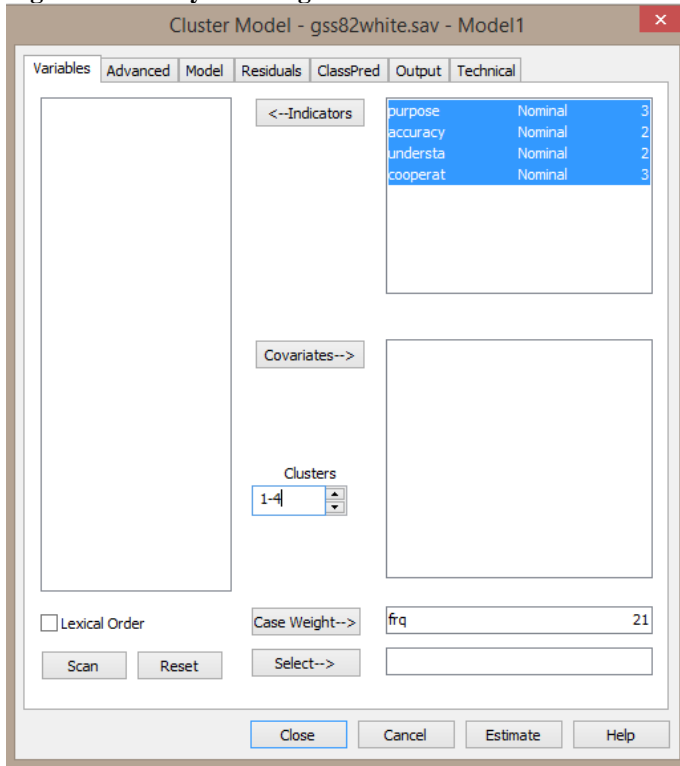
Figure 7-8. Analysis Dialog Box Prior to Model Estimation.
