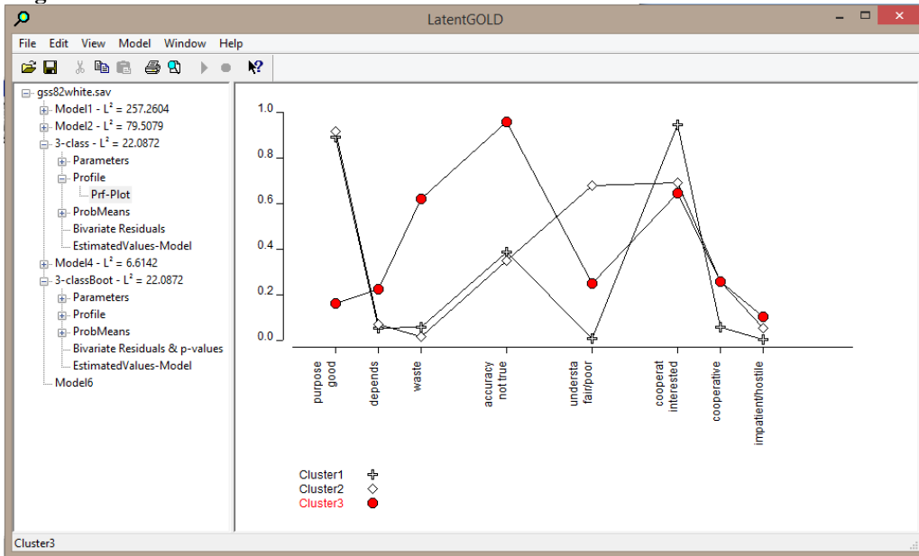
Figure 7-16. Profile Plot for 3-cluster Model
