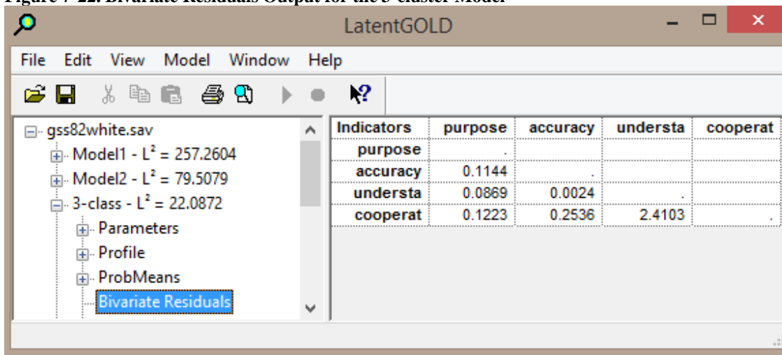
Figure 7-22. Bivariate Residuals Output for the 3-cluster Model
