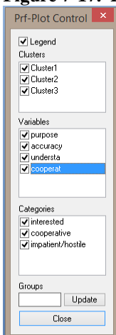
Figure 7-17. Profile Plot Control Panel
