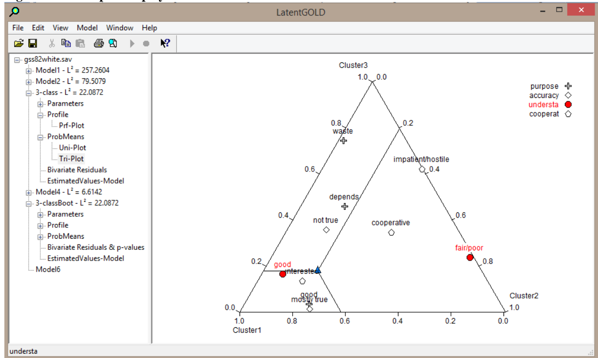
Figure 7-18. Tri-plot Display for 3-class Model
