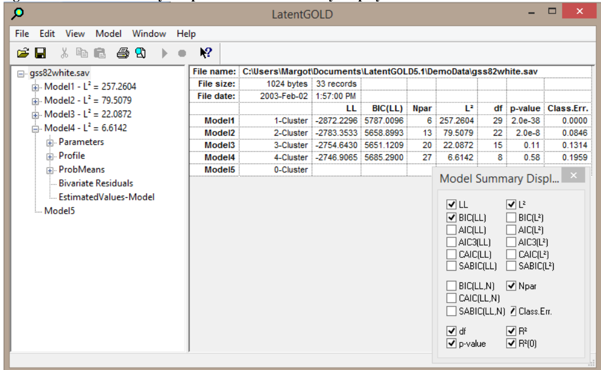
Figure 7-9: Model Summary Output and Model Summary Display
