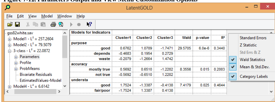
Figure 7-12. Parameters Output and View Menu Customization Options
